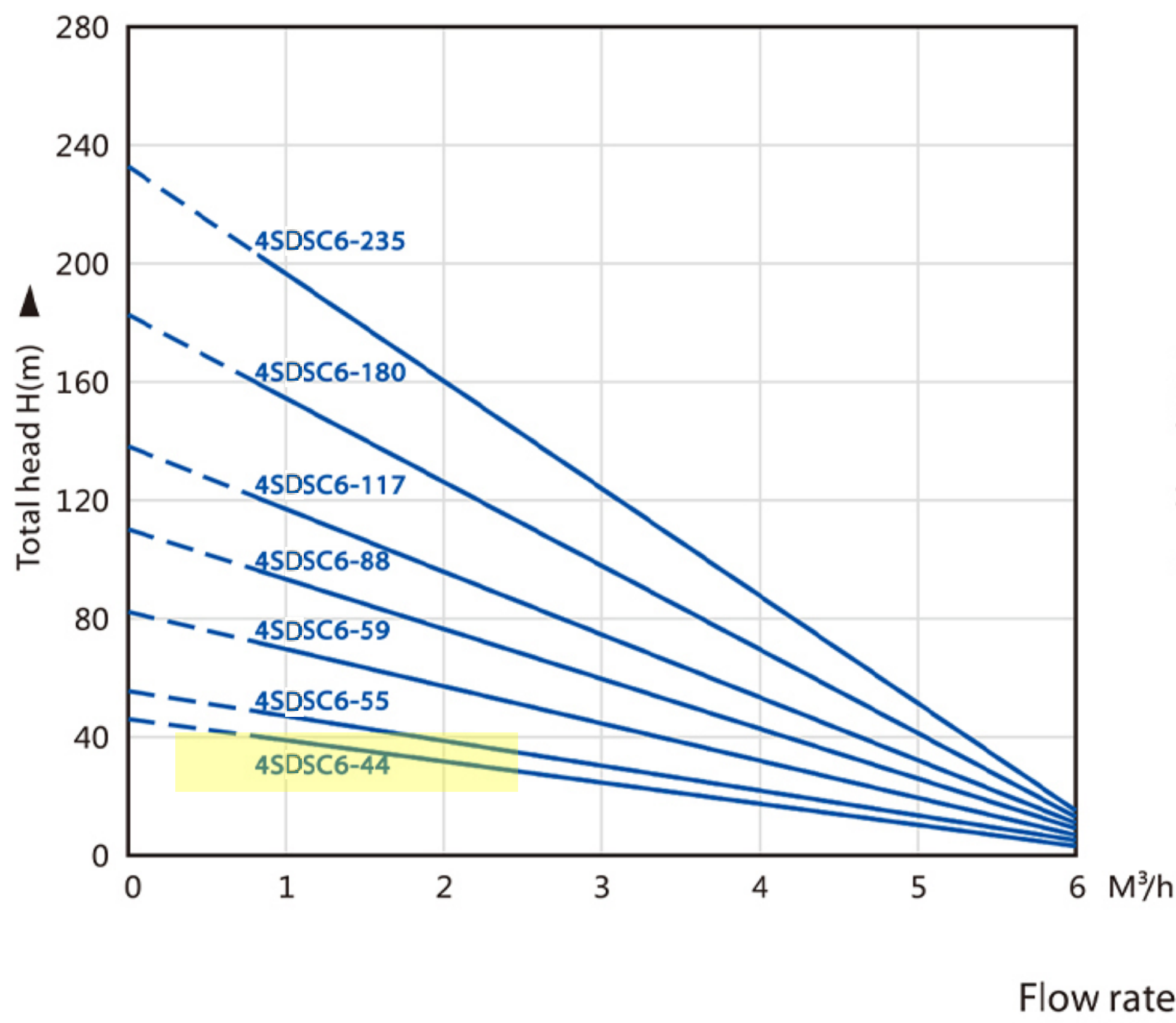
PERFORMANCE CHART AT N=4500RPM
